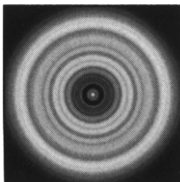
Figure 7-5 A collimated telescope should appear symmetrical with the central obstruction centered in the star's diffraction pattern.
